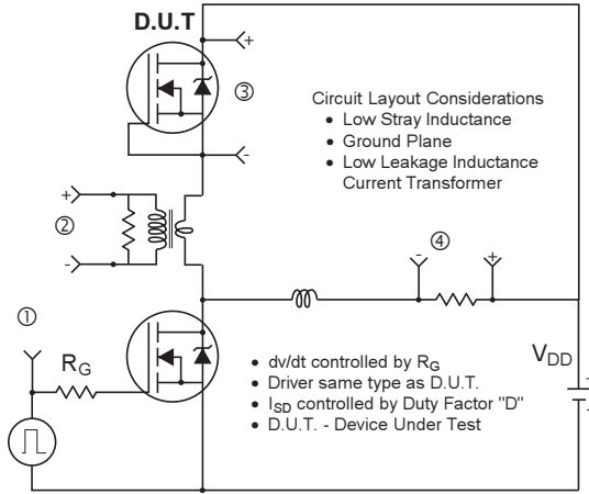
Fig 21. Peak Diode Recovery dv/dt Test Circuit for N-Channel Power MOSFETs
